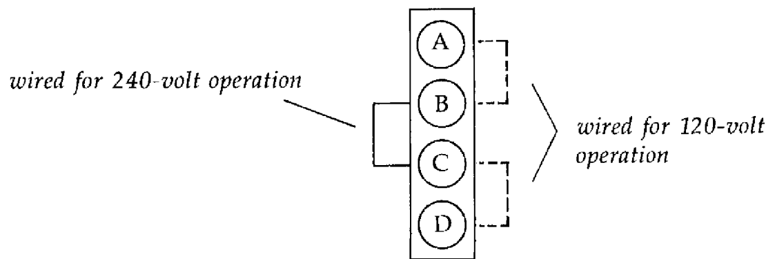
TB301 Terminal Strip
